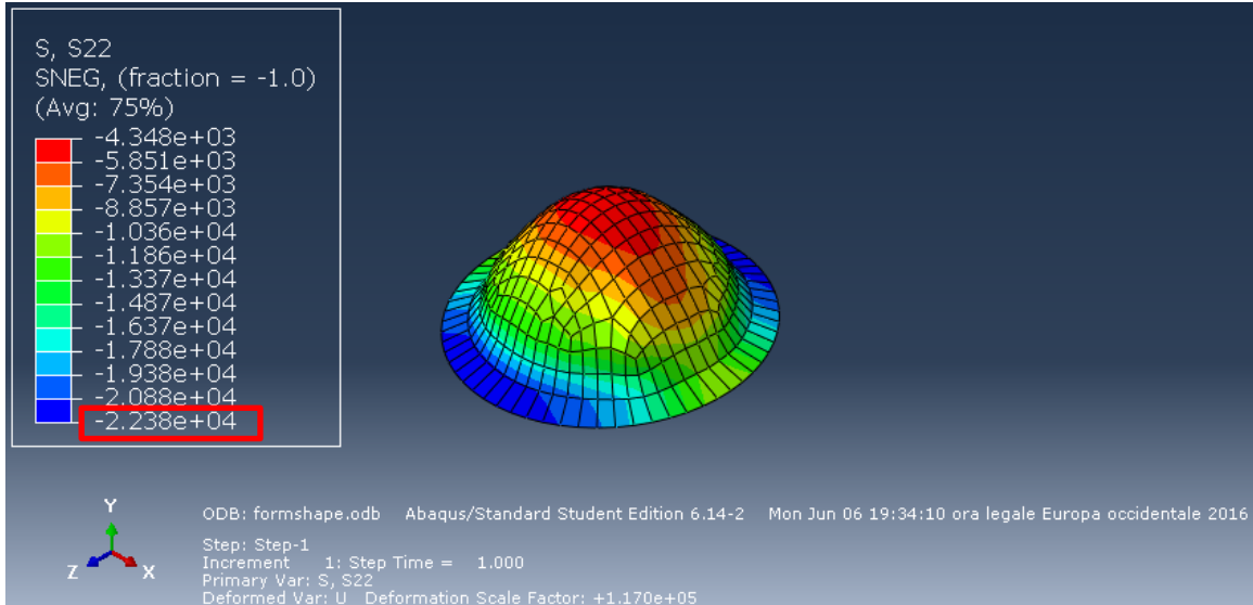
Figure 5.17. Illustration of the meridional stresses for catenoid igloo
